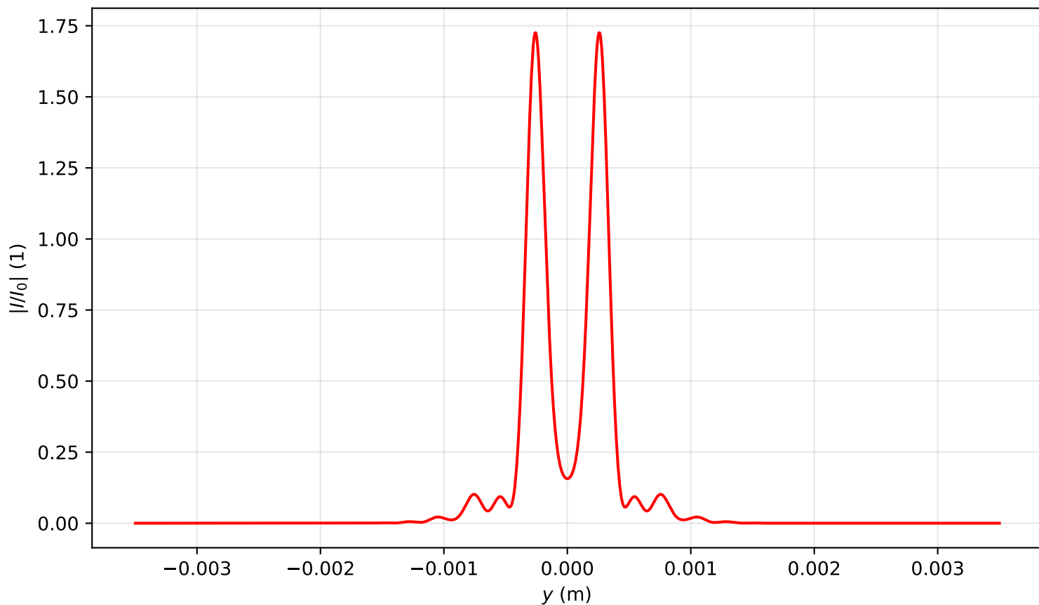
Intensity profile I(x=0, y, z=0.955)/I_0 , P_{in}=3.5P_{cr} , artificial time
